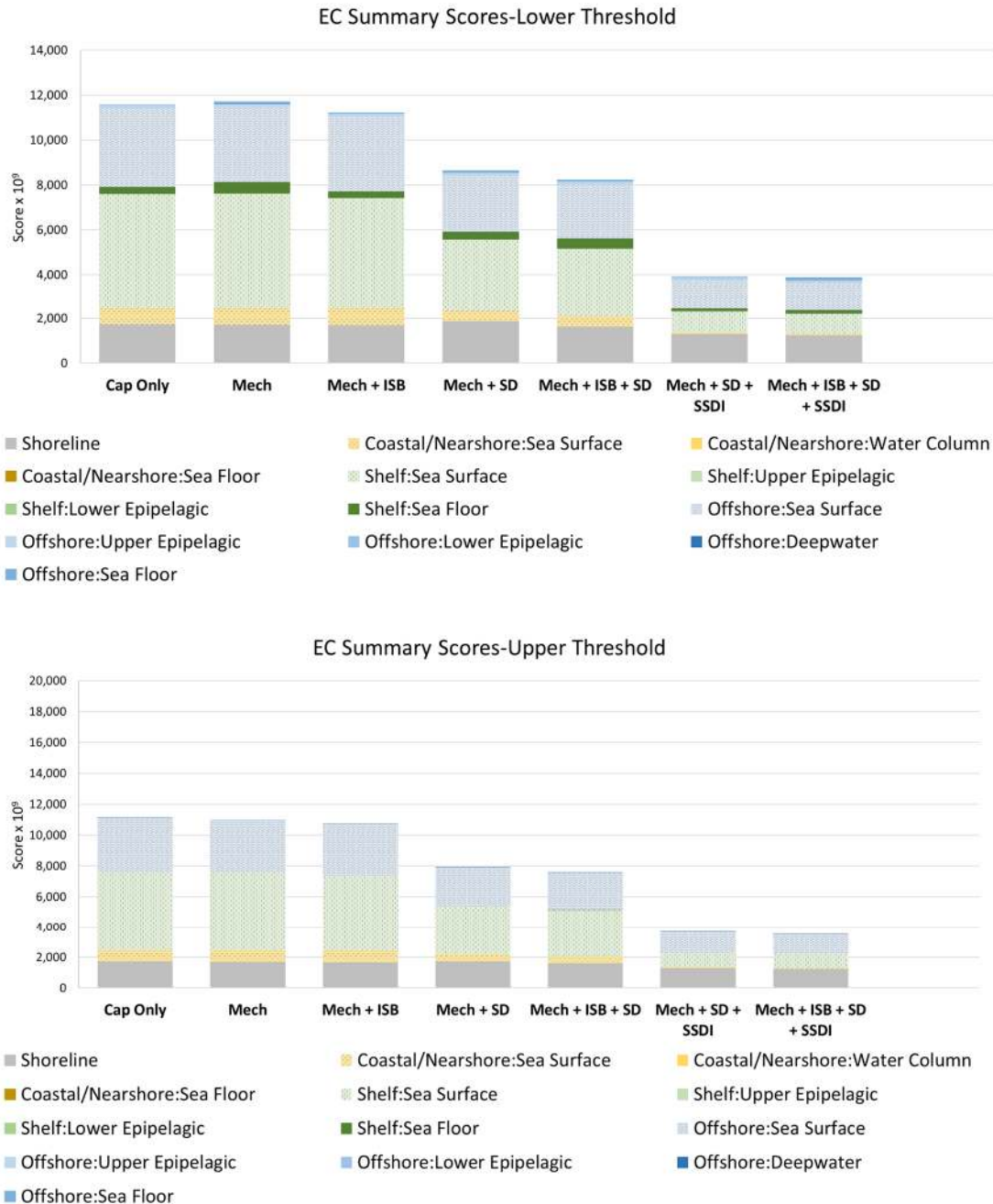
Figure 3-8. CRA Scores totaled for Environmental Compartments (ECs), applying lower thresholds (top) and upper thresholds (bottom) for ecological effects.
