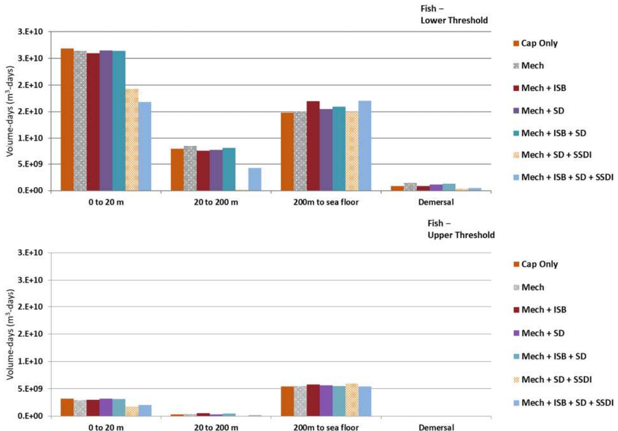
Figure 3-6. Modeled water column exposures (m³-days) exceeding a lower threshold (top) and upper threshold (bottom).
